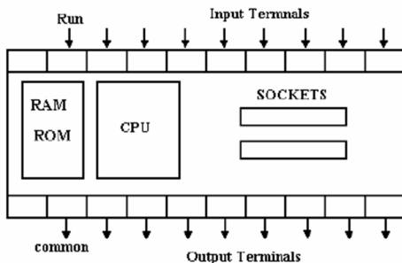
Figure 3. PLC architecture and terminology
