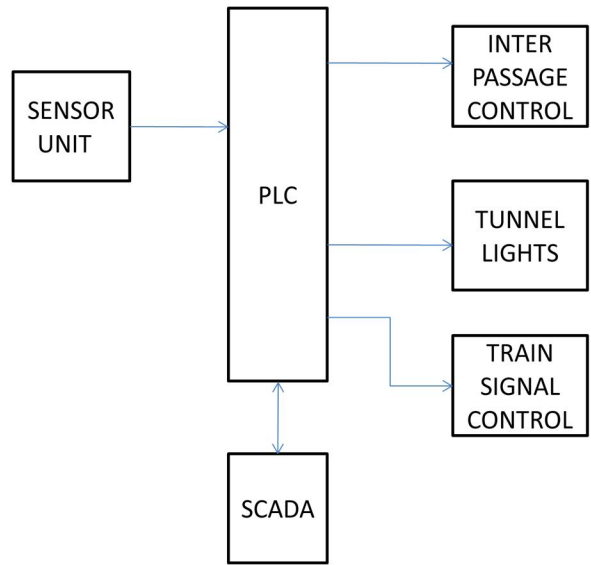
Figure1. Block Diagram for the proposed system
